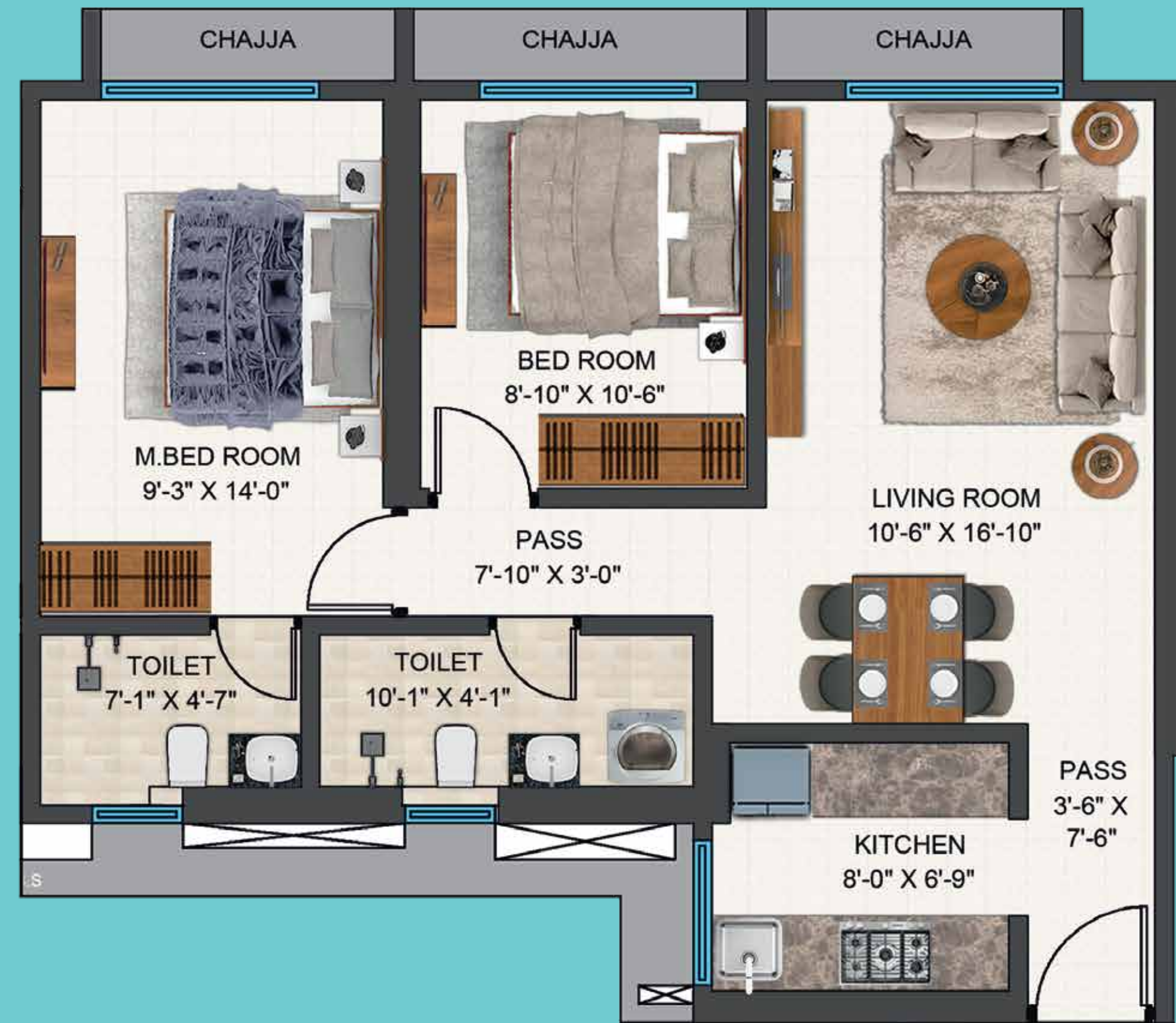
RERA Carpet Area 628.62 SQ.FT
