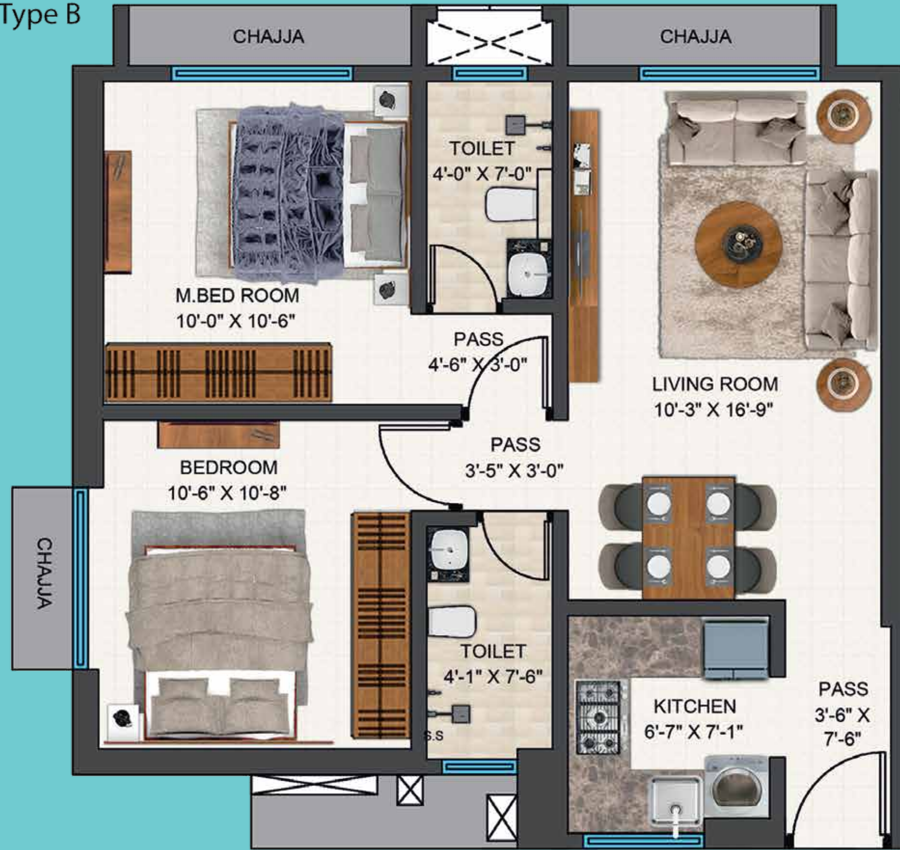
RERA Carpet Area 581.79 SQ.FT
